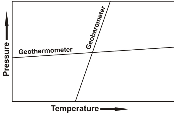
Figure 1. Diagram of P versus T (P-T diagram). Geothermometer and geobarometer are shown (notice to dips of them).
