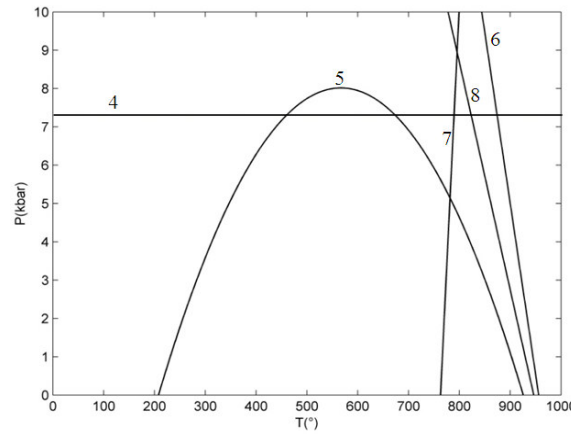
Figure 3. Exhibiting equations 4-8 for a pair coexisting Amp-Pl in an andesite [19].
