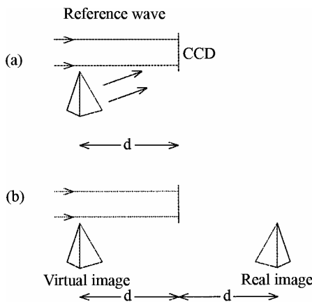
Figure 1. Digital holography (a) recording (b) reconstruction.
