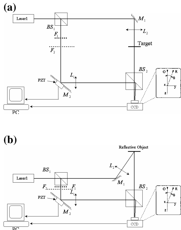
Figure 3. Geometrical arrangement for digital holography of (a) transmission object; (b) reflection object.
