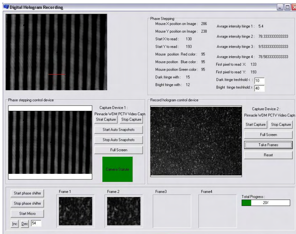
Figure 7. Calibration software.
