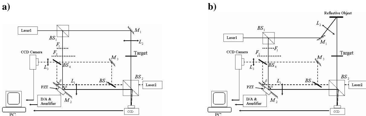
Figure 6. Geometrical arrangements for digital holography of (a) transmission object and calibration interferometer; (b) reflection object and calibration.
