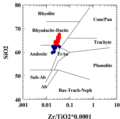
Figure 4. Classification of volcanic rocks by Zr/TiO 2 vs. SiO 2 [71]. Studied samples compositions range from Andesite, to dacite-rhyodacitic.
